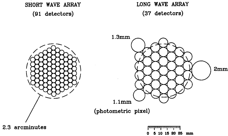
Figure 1. The pixel layout for the SCUBA arrays. The locations of the photometric pixels (1.1, 1.35 and 2.0 mm) are also shown.
