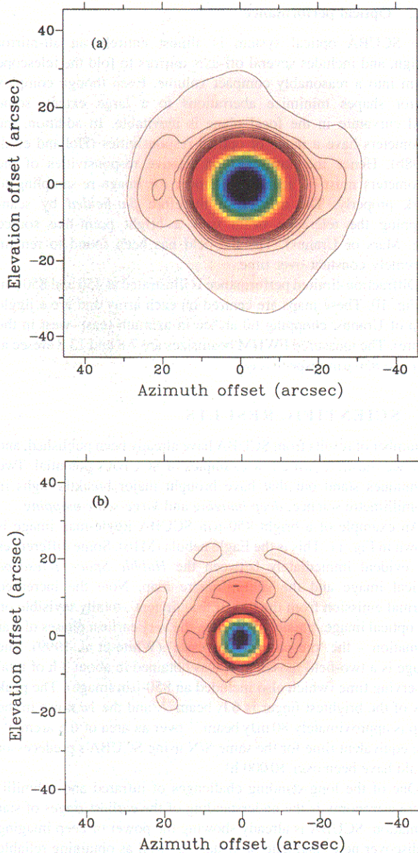
Figure 10. Beam maps of Uranus for the two array central pixels at (a) 850 \mu\text{m} (10 contours starting at 1 per cent of the peak for the base, 1 per cent intervals, and (b) 450 \mu\text{m} (2 per cent base, 2 per cent intervals).
