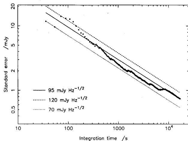
Figure 9. Standard error evolution with time for a 5-h photometry observation at 850 \mu\text{m} . Three values of system NEFD are plotted, and show that at the time of the observation the NEFD was approximately 95 \text{ mJy Hz}^{-1/2} (data are from Ivison et al. 1998a).
