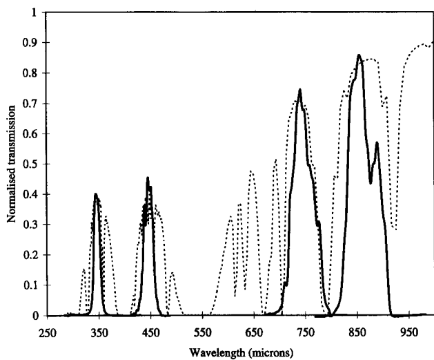
Figure 3. The measured SCUBA filter profiles (solid lines), superimposed on the submillimetre atmospheric transmission curve (dotted) for Mauna Kea for 1 mm of precipitable water vapour.
