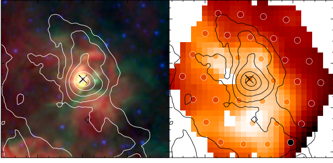
Fig. 3. Left: False-colour map of G29 showing GLIMPSE 4.5 (blue) and 8- \mu\text{m} (green) (Benjamin et al. 2003) and MAGPIS 20cm (red) (Helfand et al. 2006). Right: [N II] line flux towards G29. The circles show the position of the bolometers on the sky. The space between them has been interpolated using inverse distance weighting. The X marks the position of the G29.96-0.02 radio source (Wood & Churchwell 1989, 18^{\text{h}}46^{\text{m}}03.96^{\text{s}} , -02^{\circ}39'21''.5 ). The diamond marks the position of the NII peak. The contours are SCUBA 850 \mu\text{m} emission (5, 10, 20, 50 and 100 times the local off-source rms) showing the extent of the G29.956-0.017SMM clump.
